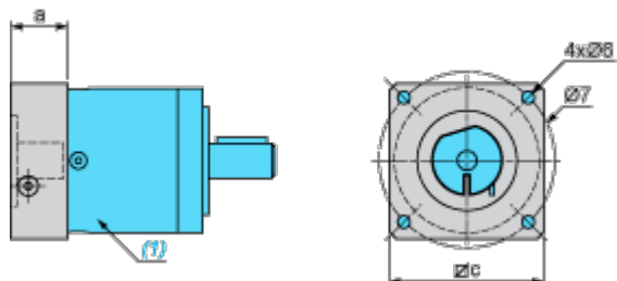
(1) Gearbox
